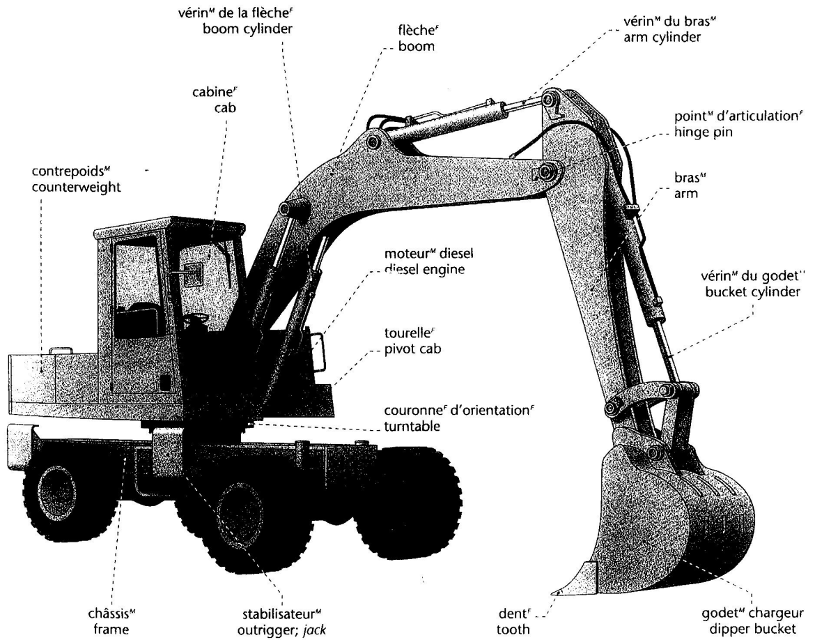
PELLE f HYDRAULIQUE HYDRAULIC SHOVEL
